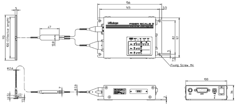
Dimensions of Processor
