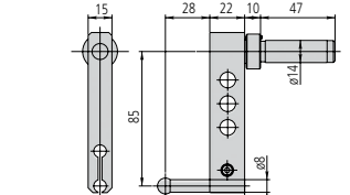
12AAA793 Probe extension holder (85mm/3.3")
