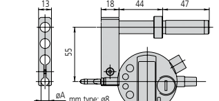
12AAA837 Dial indicator (ø3/8" stem) holder
