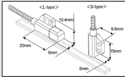
Dimensions of Detector Heads
