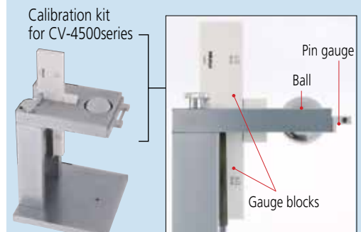
Calibration Kit: CV-4500: 12AAQ491 CV-3200: 12AAQ489 (not shown)
